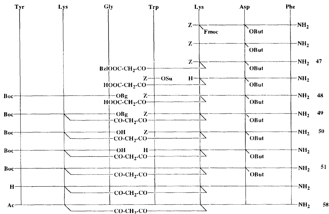
Figure 3. Synthesis of compound 58 .
