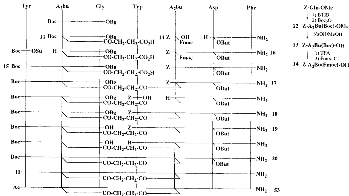
Figure 2. Synthesis of compound 53 .
