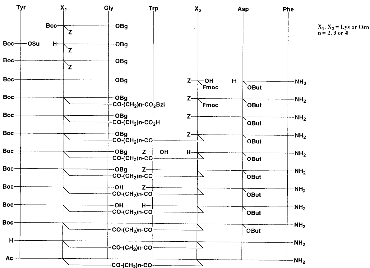
Figure 1. Synthesis of compounds 52 , 54–57 , 59 .
